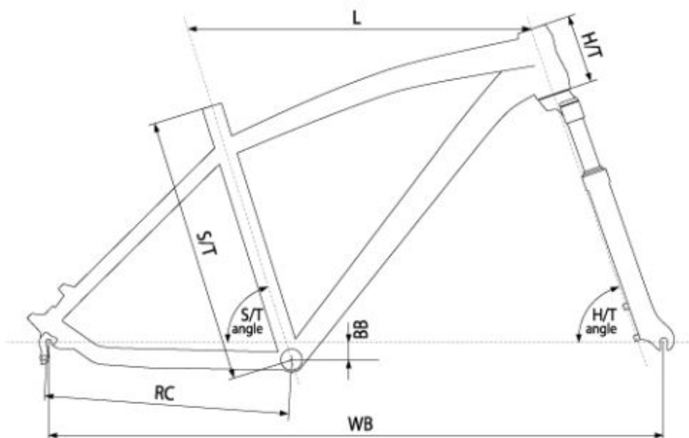
HARDTAIL: Kellys 6Box SWT 6061 triple butted - Race Geometry
