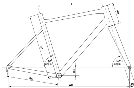
ROAD: KELLYS Endurance Concept - Aluminium alloy
