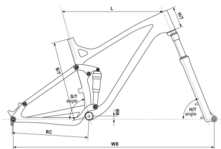
MOUNTAIN - ENDURO: KELLYS Enduro High-modulus Carbon Composite monocoque 27.5
