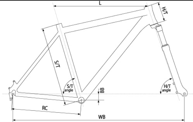
HARDTAIL: Kellys Alutec Lite 6061 triple butted - RRCG (Race Ready Concept Geometry)
