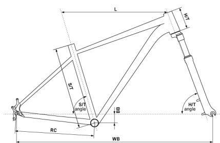
MOUNTAIN - MTB-XC: KELLYS Alutec RRC 27.5
