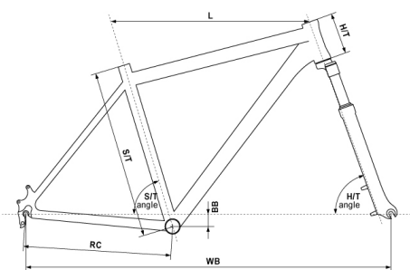
MOUNTAIN - MTB-XC: KELLYS Atutec RRC 27.5
